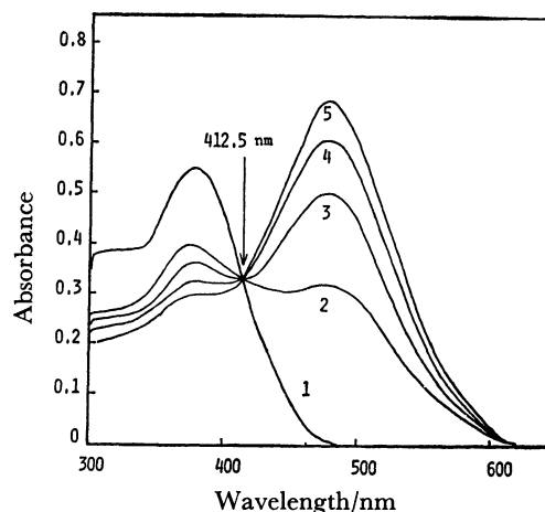
Fig. 1. UV spectra of \text{BuNH}_2\text{-HA-18C6} system.
